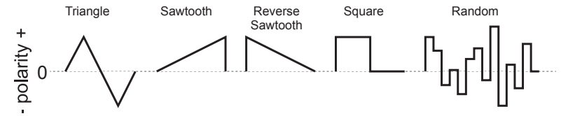
LFO waveshapes
